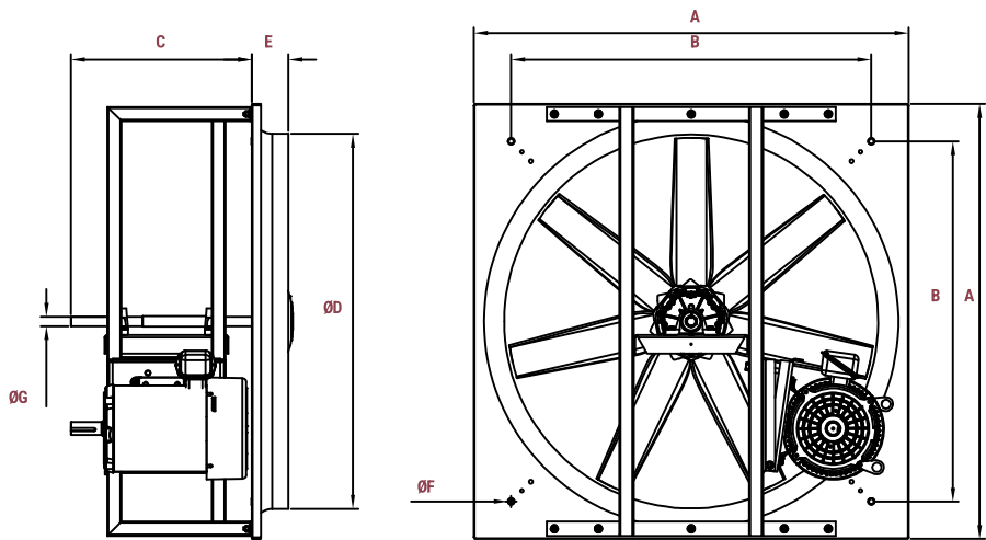
EXTRACTOR HGTA
