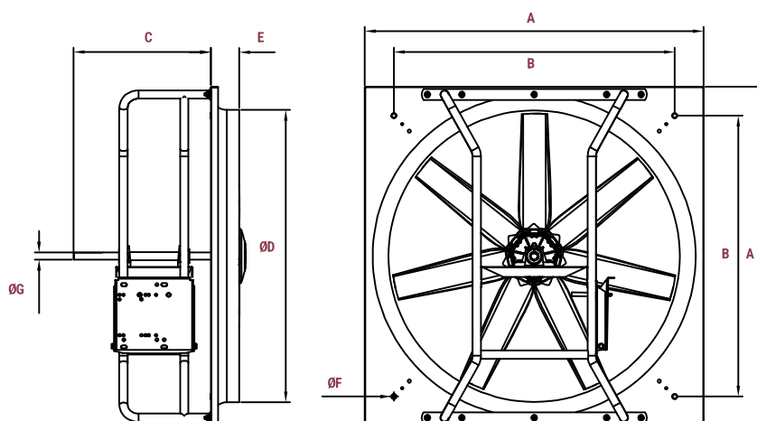
EXTRACTOR HGTA
